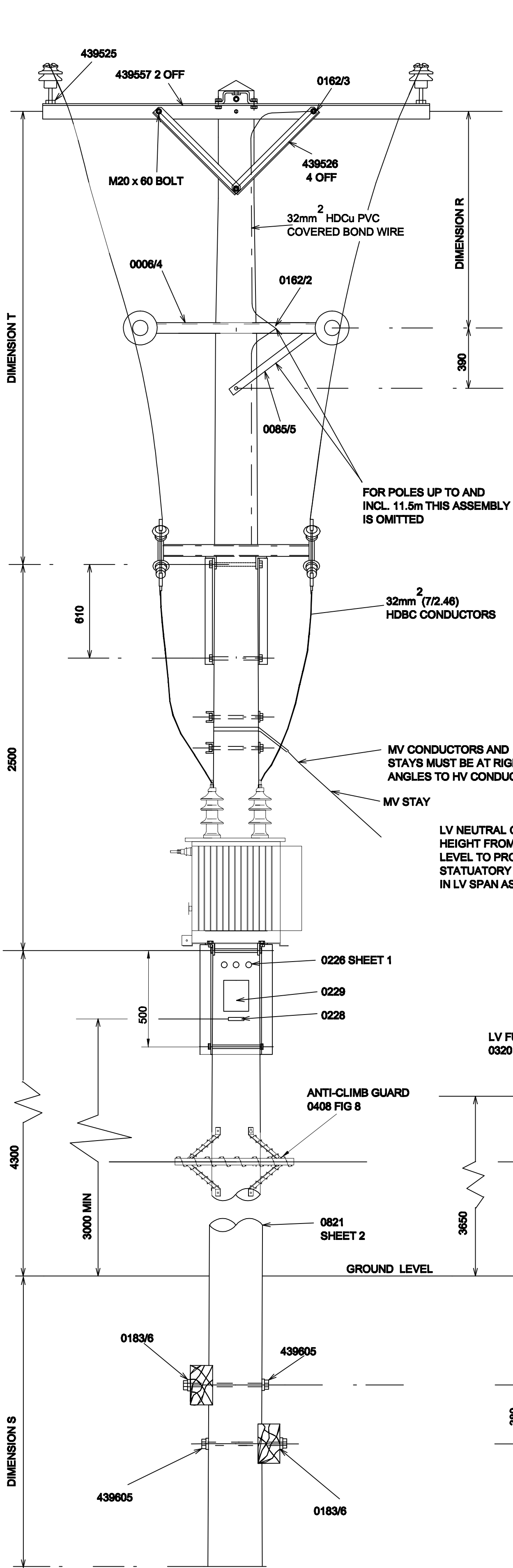
FIG 1 PLATFORM MOUNTED TRANSFORMER IN LINE ARRANGEMENT
